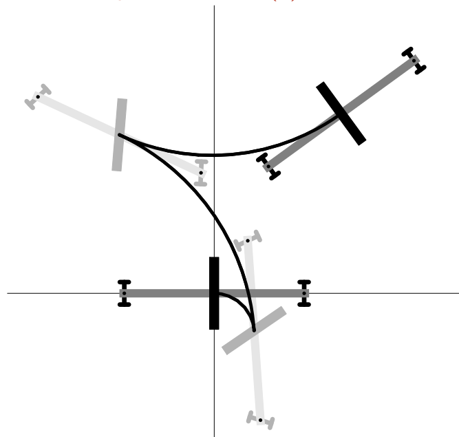
snakeboard as \Sigma_2 -system
